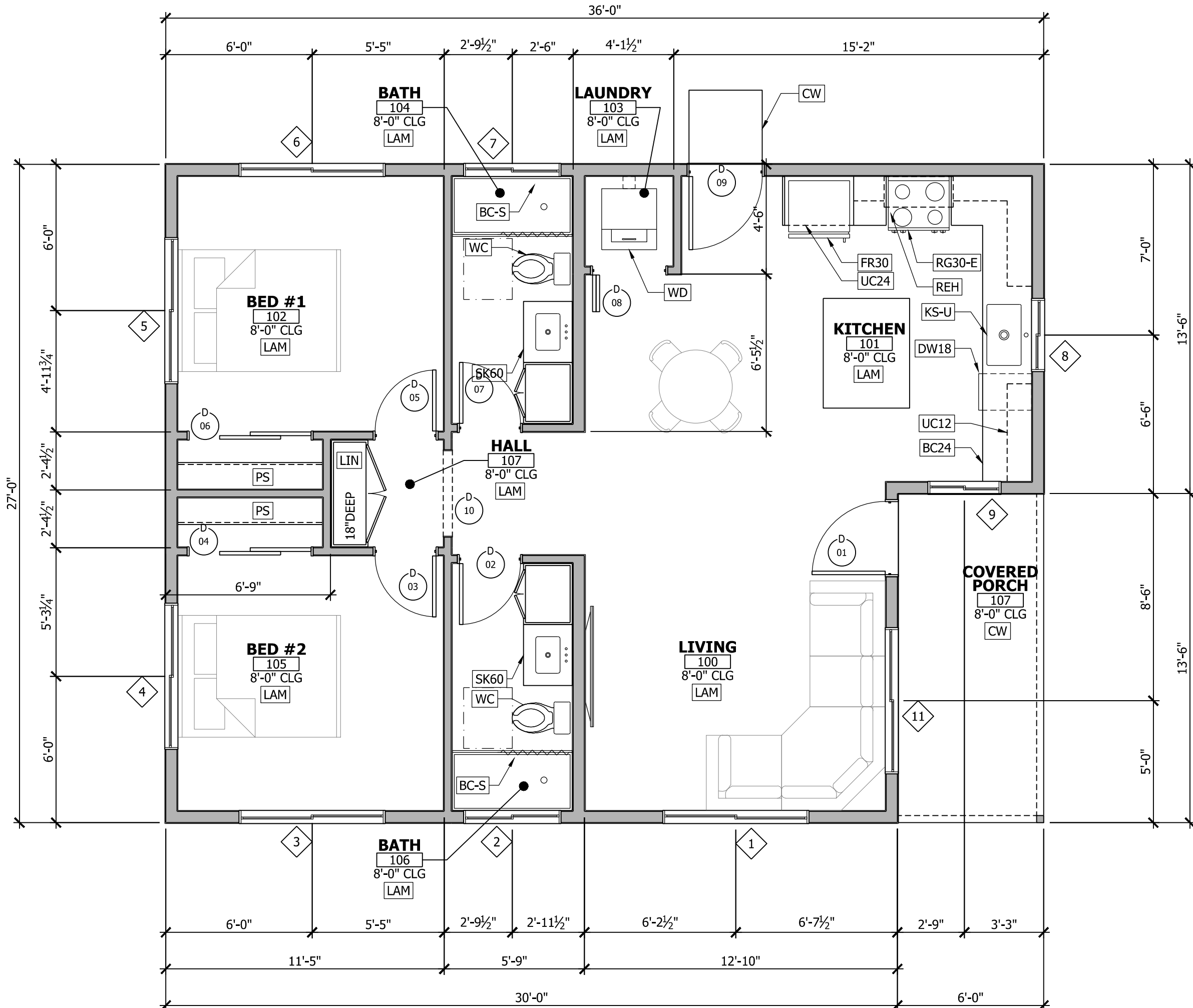
1 FLOOR PLAN
